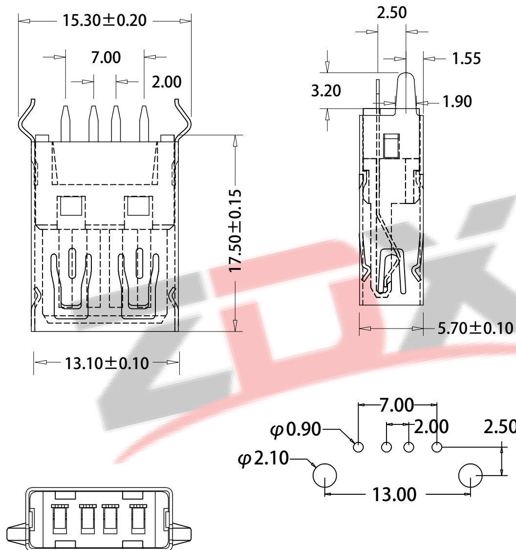
RECOMMENDED P.C.B LAYOUT
