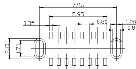
RECOMMENDED PCB LAYOUT(t=0.80±0.05) COMPONENT SIDE(GENERAL TOLERANCE±0.05)
