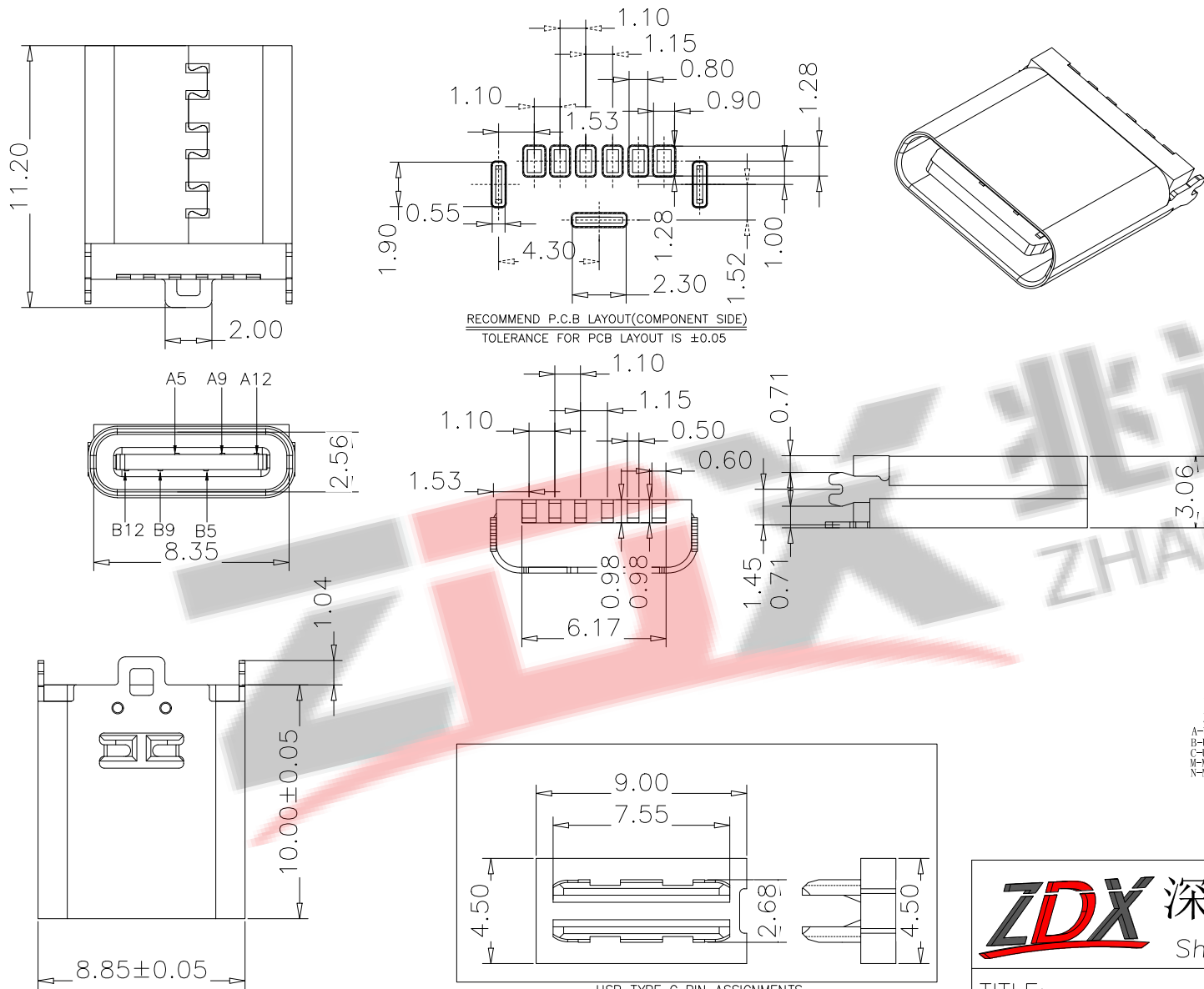
USB TYPE C PIN ASSIGNMENTS
