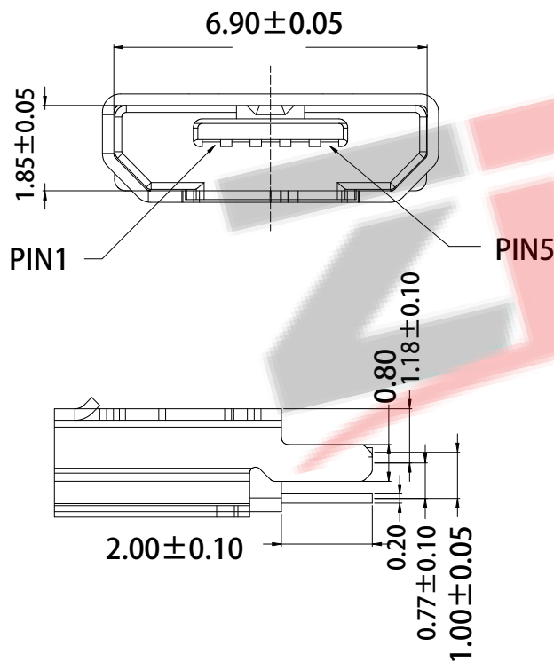
MICRO USB B TYPE PIN ASSIGNMENTS
